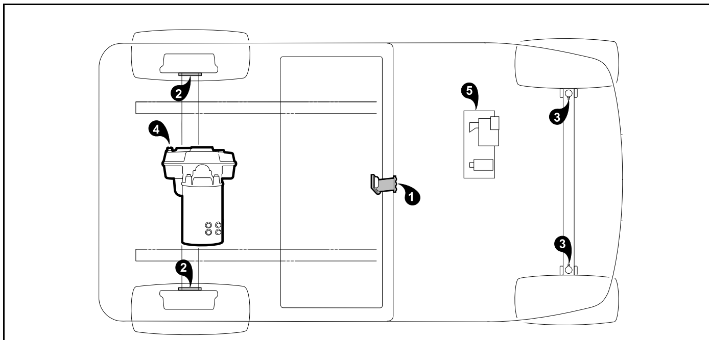
64 Figure 23 Lubrication Points – Electric Vehicles
