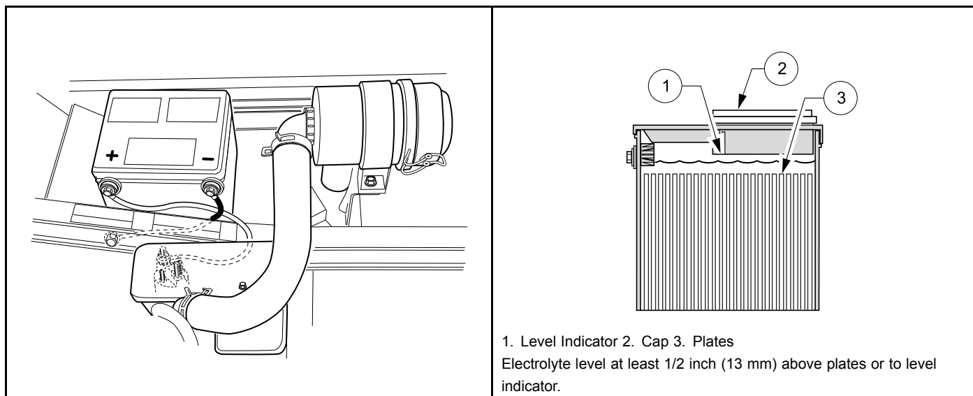
2831 Figure 33 Side-Post Battery- Gasoline Vehicle Battery
